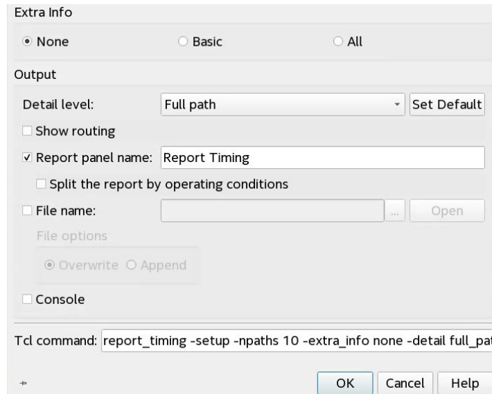
Figure 39. Report Timing Dialog Box (Bottom Section)
